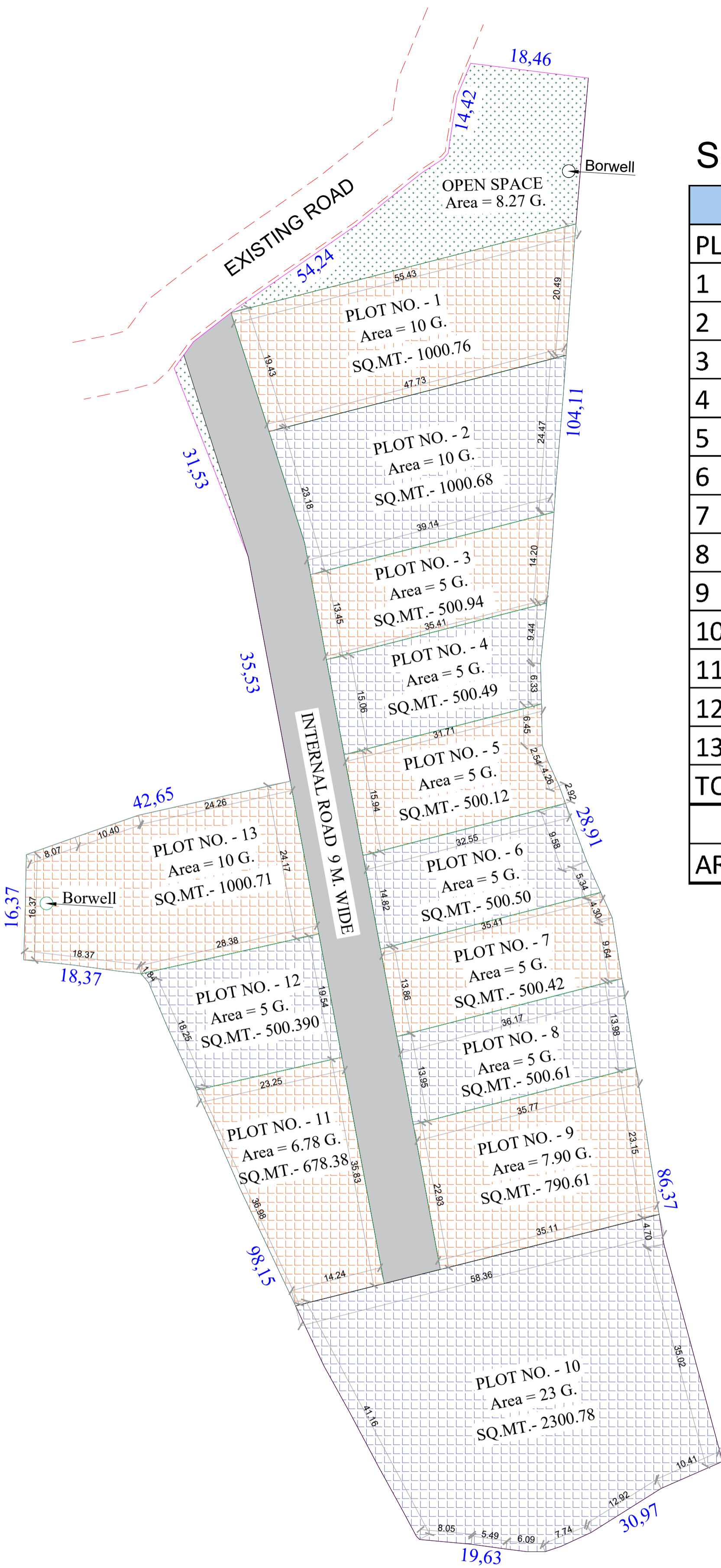
LAYOUT PLAN
